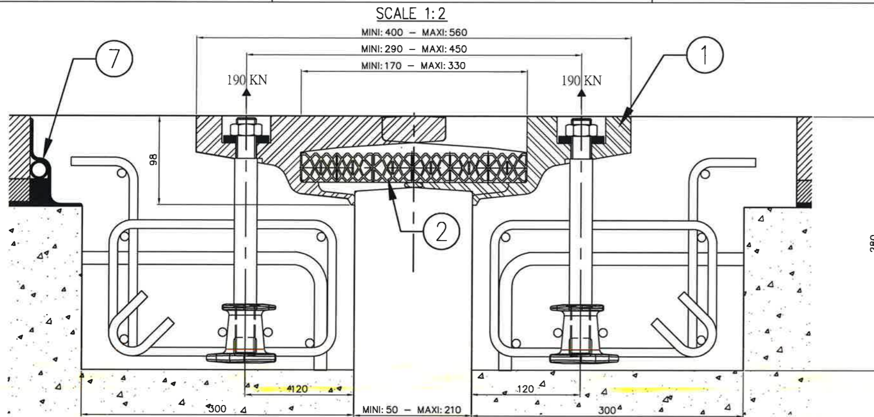
SCALE 1:2 METALLIC ELEMENTS 998
