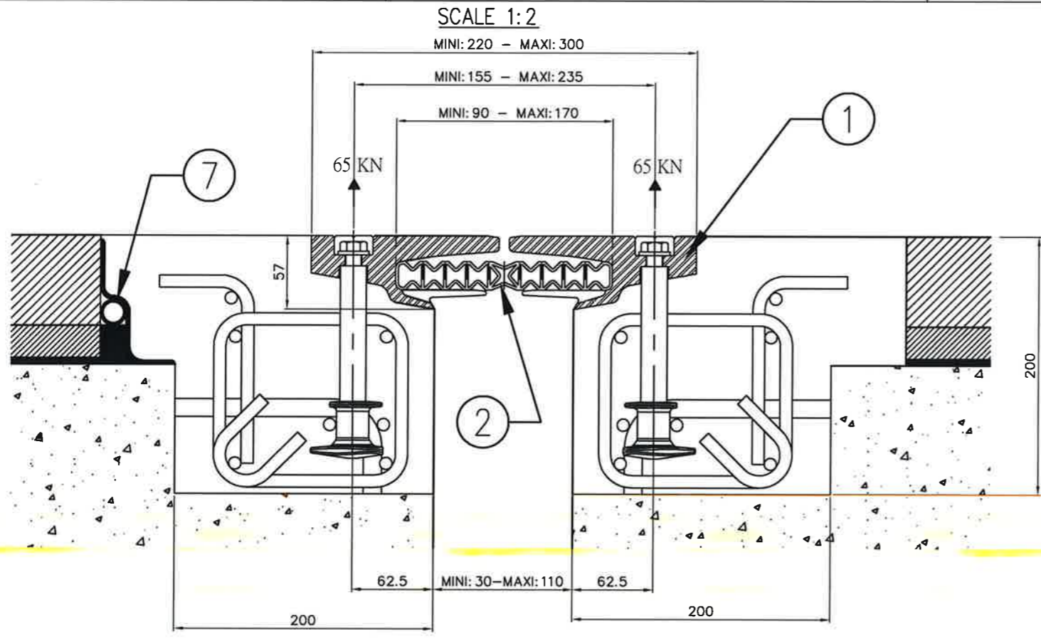
SCALE 1:2 METALLIC ELEMENTS
