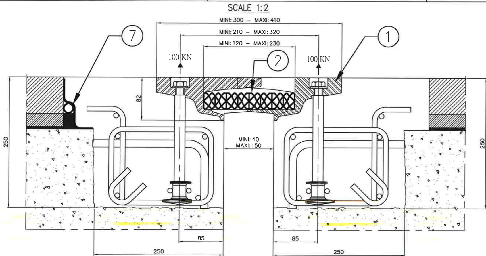
SCALE 1:2 METALLIC ELEMENTS 998
